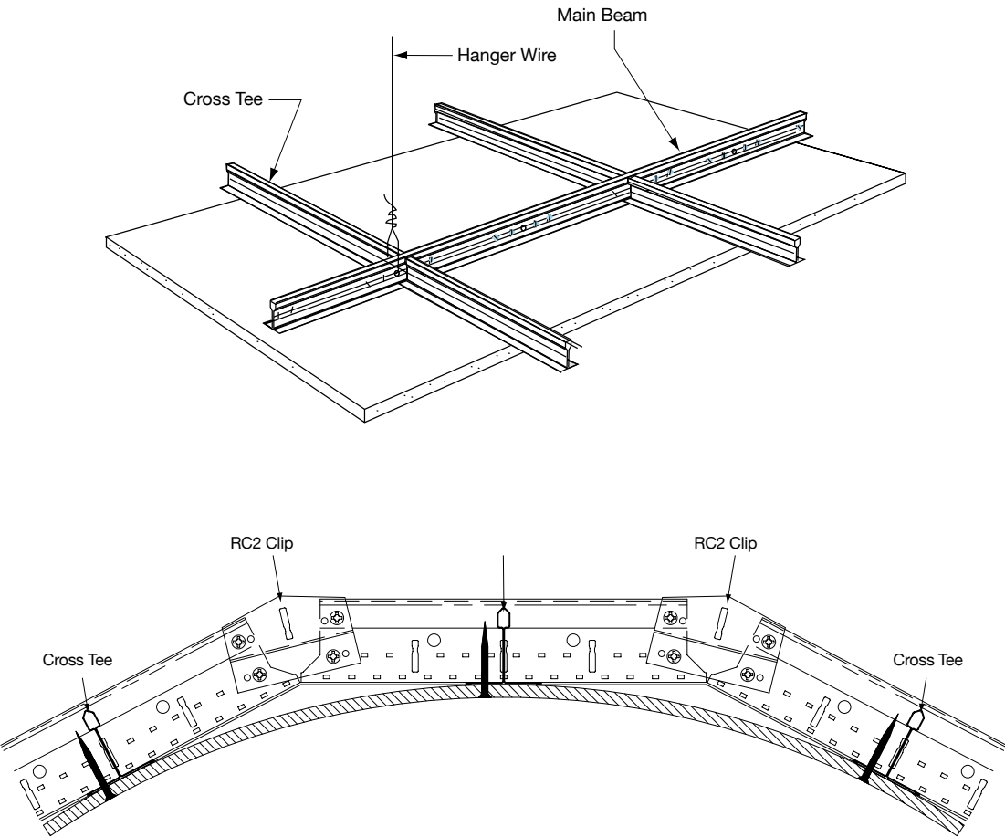
Drywall Grid System for Flat and Curved Drywall
