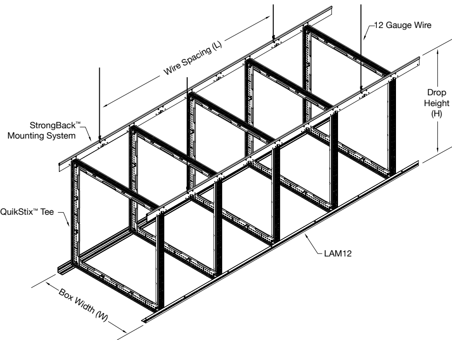
Quikstix™ Drywall Soffit Framing System
