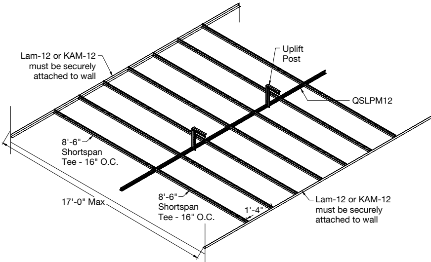
ShortSpan® Drywall Framing System
